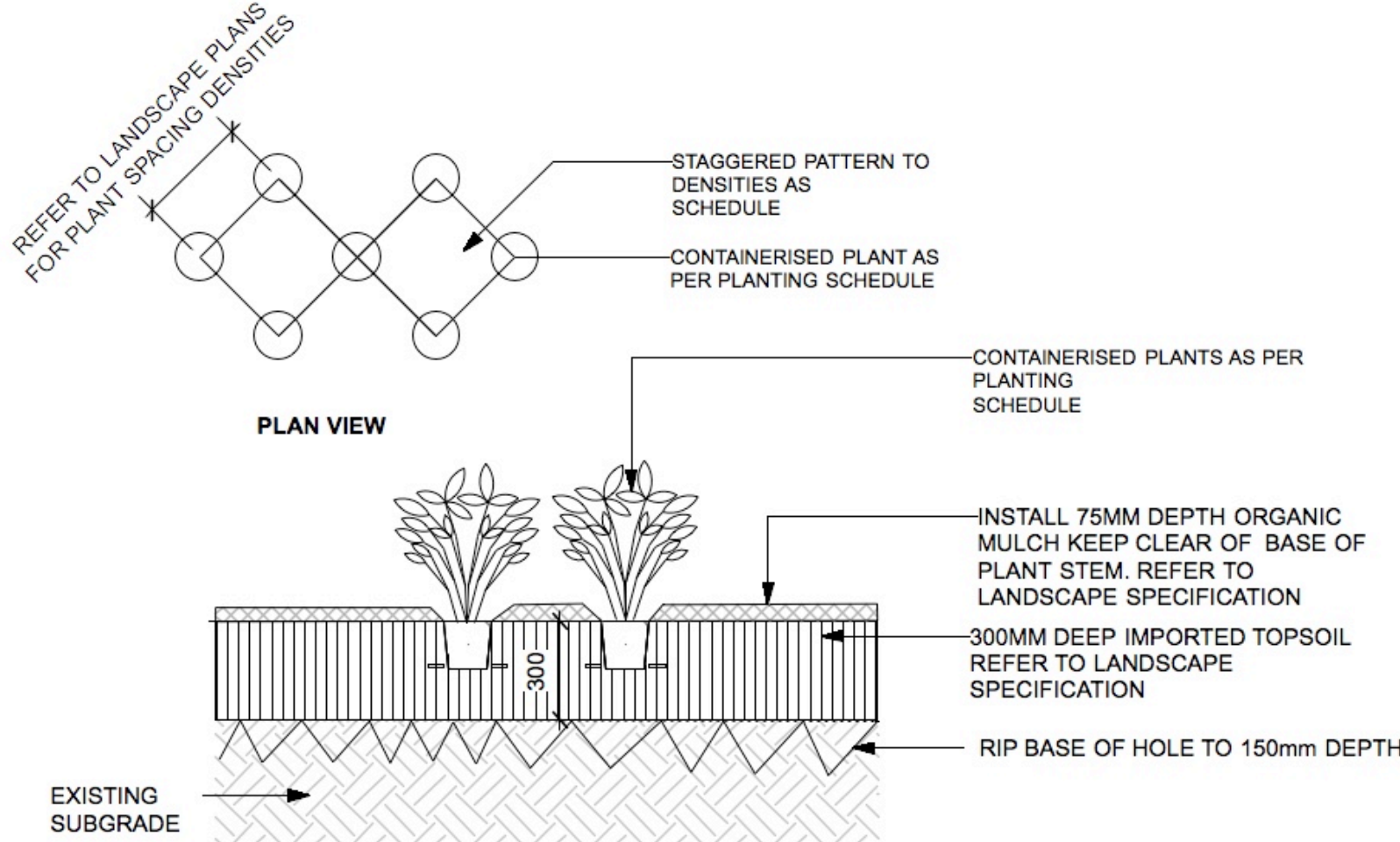
TYPICAL GROUNDCOVER PLANTING DETAIL SCALE 1:20
