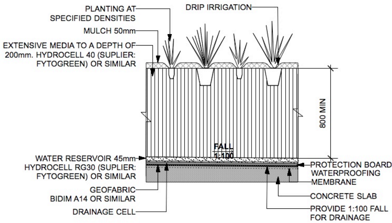
TYPICAL PLANTING ON SLAB DETAIL (Groundcovers to Medium Sized Trees) SCALE 1:20
